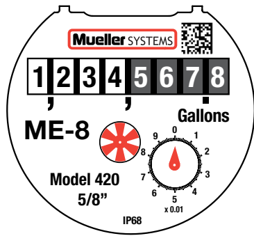
MODEL 420, 435, 452
