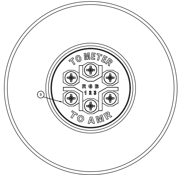
TRuRead Rear Connection View
