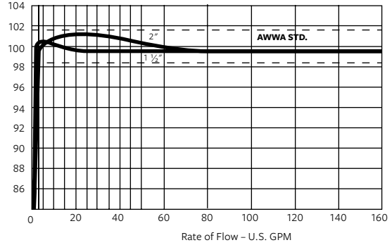
Accuracy - 1 \frac{1}{2} " and 2"
