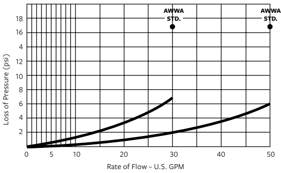
Head loss - \frac{3}{4} " and 1"
