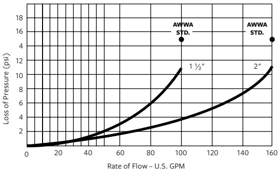
Head loss - 1 \frac{1}{2} " and 2"
