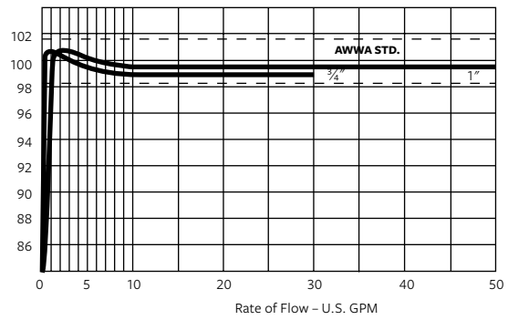
Accuracy - \frac{3}{4} " and 1"
